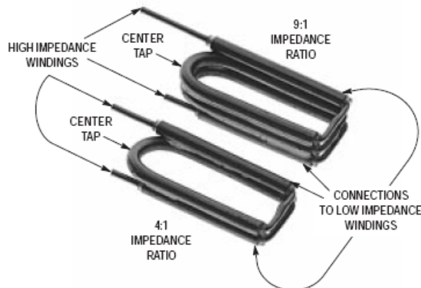
Figure 6. RF Transformer
