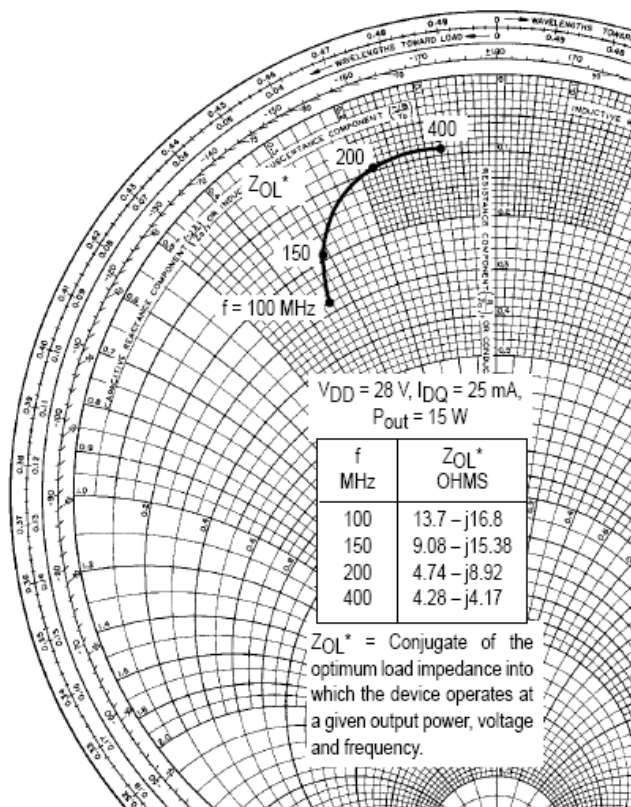
Figure 17. Large-Signal Series Equivalent Output Impedance, Z_L^*
